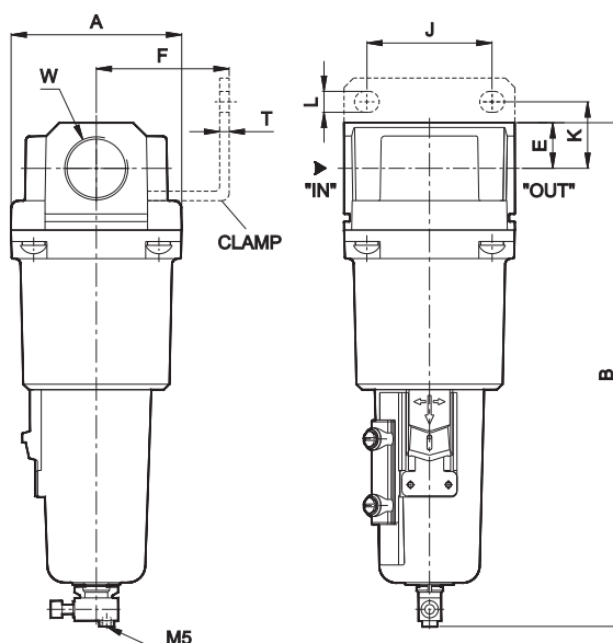
Model F17....-LM
