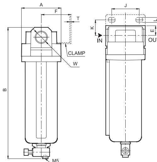
Model F17....-LM
