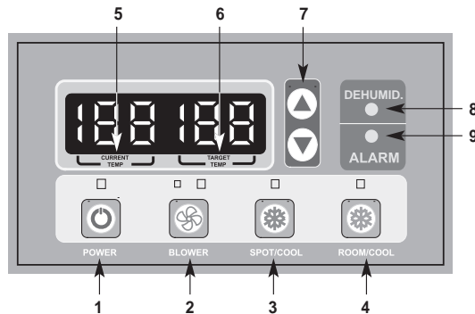
Figure 21 - Display/Control Panel
